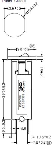
Panel Cutout
