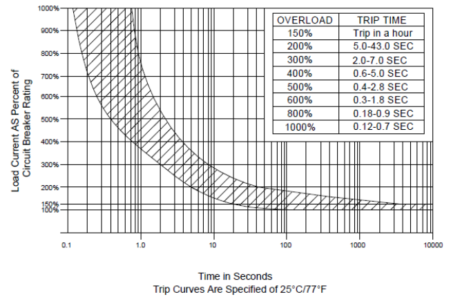
Trip Time Curves
